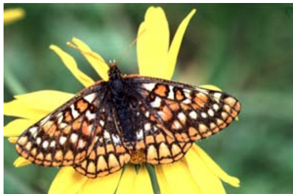
Figure 1. Adult Cloudcroft checkerspot butterfly. observed in late July, 1997. Photo by J. Popp.
