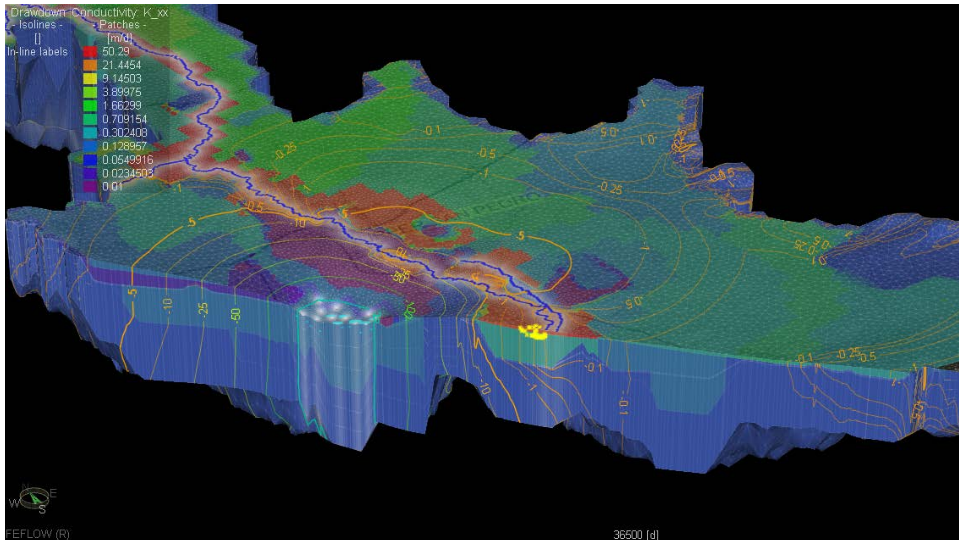
Figure 21. Simulated Drawdown (m) in cutaway through Vigneto Development (refined grid in the center) and Saint David Cienega (yellow symbols). Lowest model layer shown represents a 500 m thick weathered bedrock zone, using 0.01 m/d conductivity. Results clearly show that drawdown from Vigneto pumping is largely damped due to the higher permeability flood plain deposits, colored lighter red here, adjacent to the San Pedro River. Still, water levels beneath the Saint David Cienega area decline about 1 foot.
