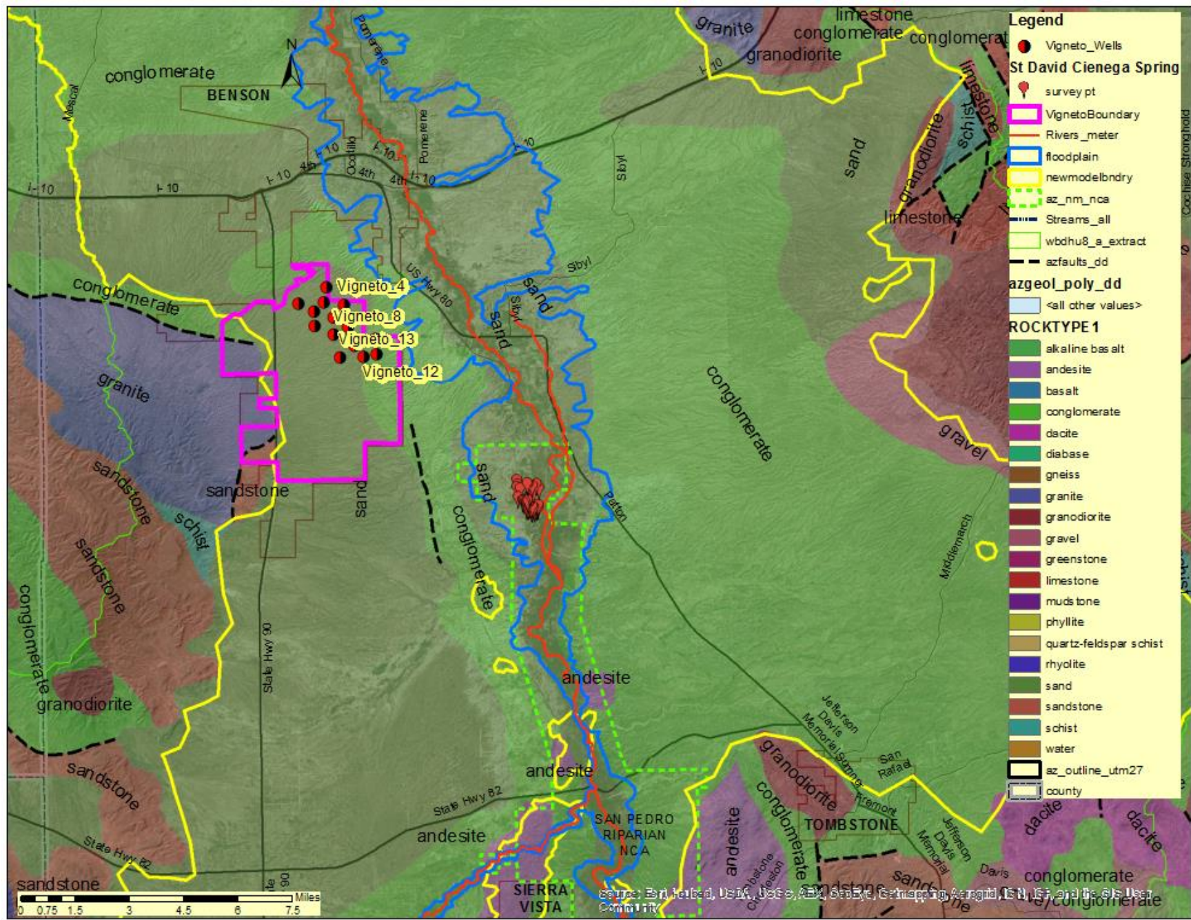
Figure 6. Surficial Geology (Arizona USGS). San Pedro River National Conservation Area is shown in dashed green line (same as az_nm_nca in legend).
